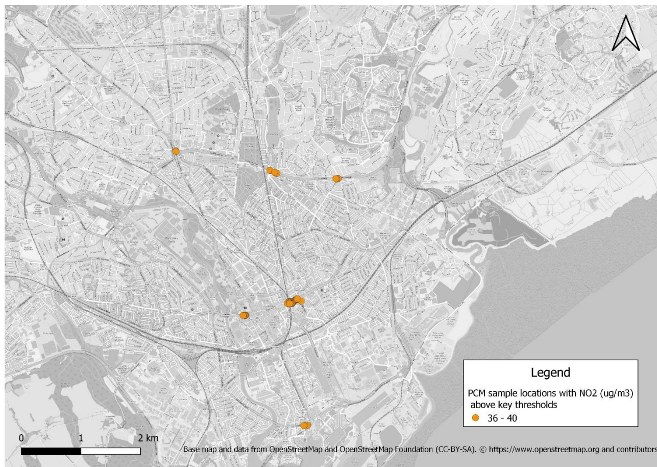
Figure 5-2: PCM receptors with NO 2 concentrations above desired thresholds (2022 baseline)
